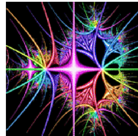
th_fractals-14
